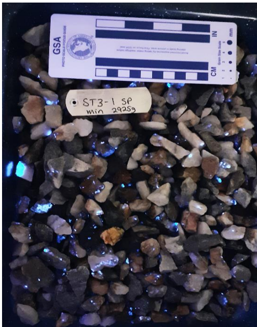
Figure 1 - XRT Sorter Product with scheelite under ultraviolet lamp
